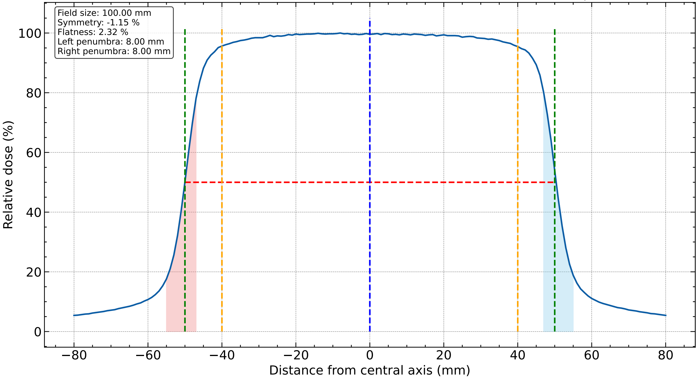
10MV, Beam Profile(Crossline), SSD=100CM, F.S=10X10 cm 2 , Depth=10cm
